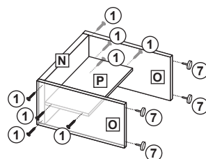
Step 4 (Chair Part)
